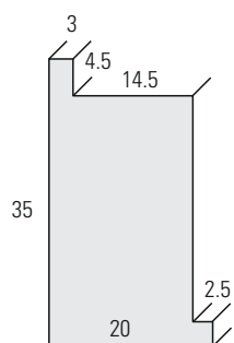
20.5250.35 LI
