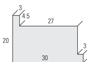
30.5250.20 LI
